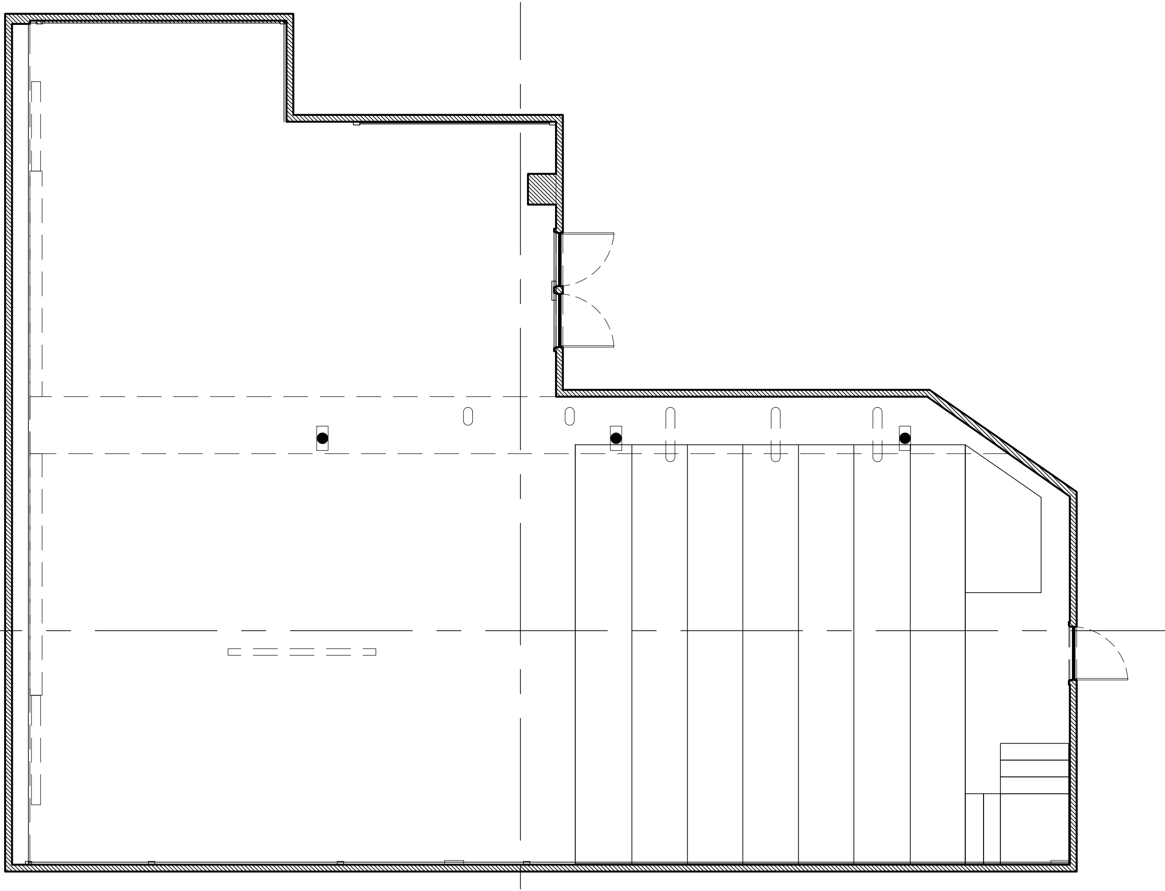
THE DEN THEATRE MAINSTAGE GROUNDPLAN SCALE: \frac{3}{16}'' = 1'0''
